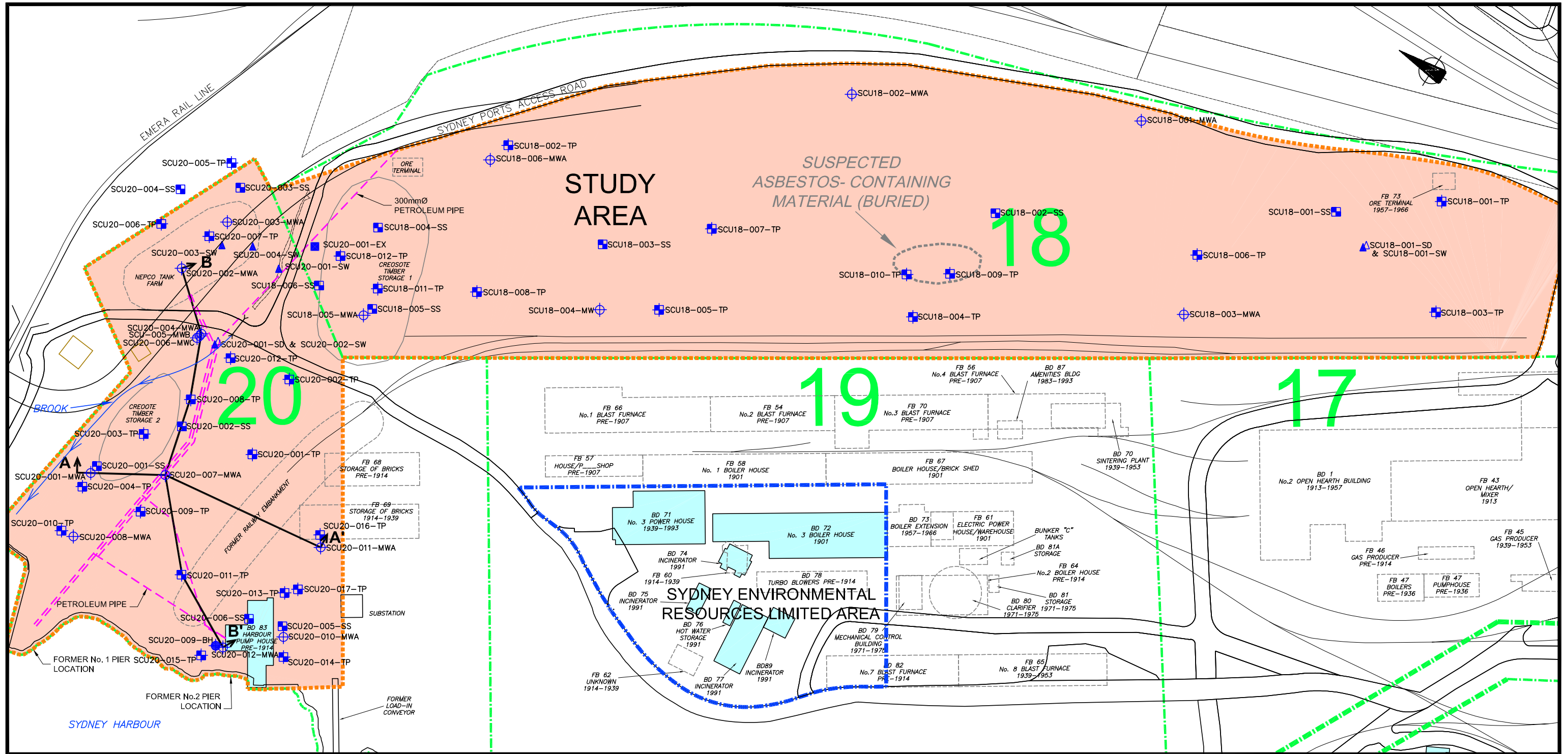
FIGURE 2 SAMPLING LOCATION PLAN SCALE 1:2000 (APPROX.) ERNST & YOUNG INC. c/o SYSCO PHASE II ENVIRONMENTAL SITE ASSESSMENT/No. 1&2 PIERS AREA BLAST FURNACE STOCKYARD, SYDNEY, NS TV23209
